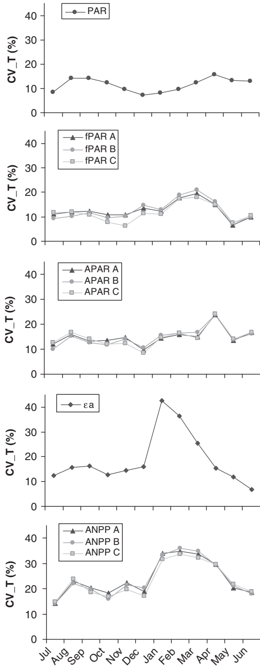
Fig. 6. Temporal (among years) variability in monthly values of the considered variables expressed as the coefficient of variation (CV_T). PAR: incident photosynthetically active radiation; fPAR: fraction of photosynthetically active radiation absorbed by green vegetation; APAR: photosynthetically active radiation absorbed by green vegetation; εa: energy conversion coefficient of absorbed radiation into aboveground biomass; ANPP: aboveground net primary production; (a) Meso-xerophytic grasslands; (b) Lithophytic steppes; (c) Meso-hydrophytic grasslands. fPAR, APAR and ANPP values are averages for all pixels in each unit.
